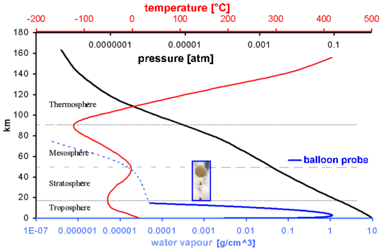
Fig. 1: Structure of the Atmosphere (Source: ESPERE)
